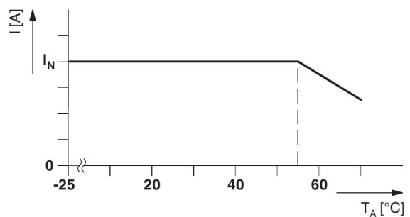
Figure 14 Temperature-dependent derating
