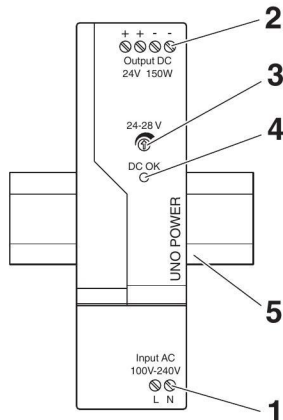
Figure 1 Device elements
